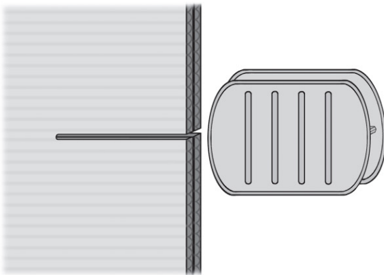
Interlock 'H' Clip before locking
